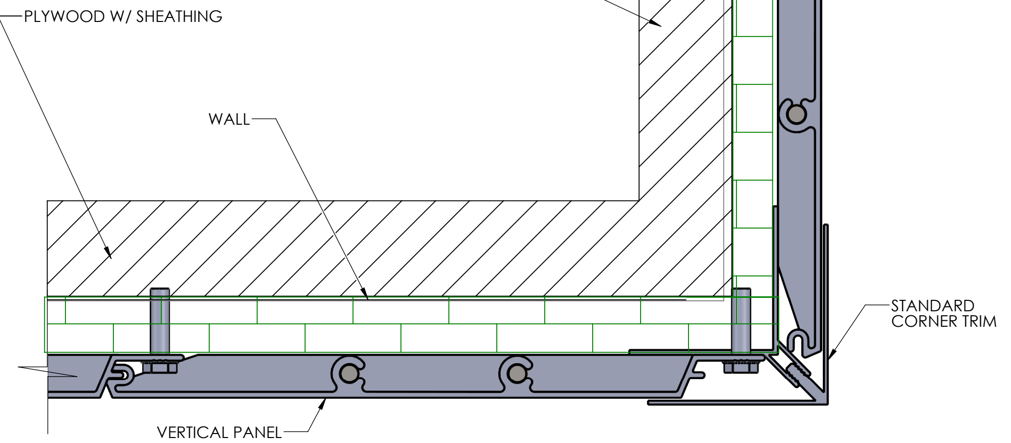
STANDARD CORNER SECTION WALL SECTION
